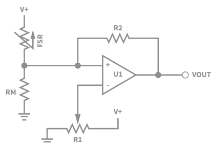
Figure 10. Force-Sensing Resistor Variable Force Threshold Switch
