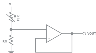
Figure 8. Voltage divider.
